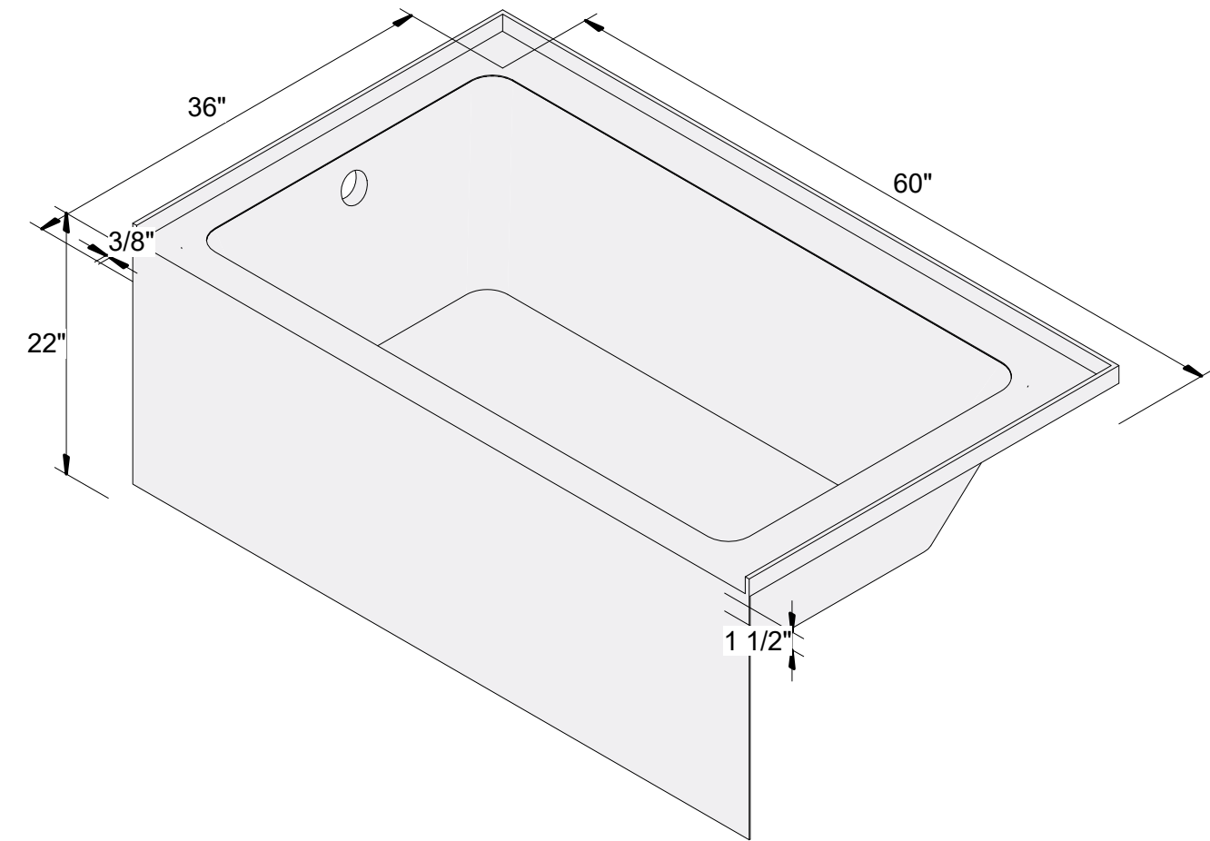
ISO VIEW
