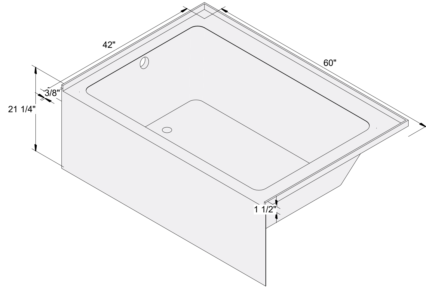
ISO VIEW
